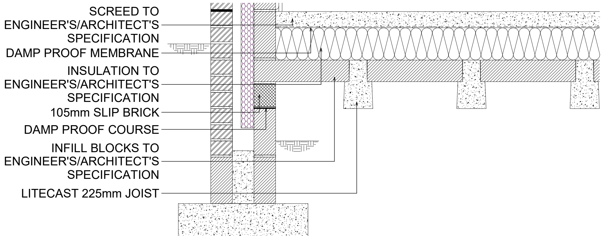
TRADITIONAL 225mm BEAM AND BLOCK SOLUTION TYPICAL CONNECTION WITH TRADITIONAL MASONRY WALL
