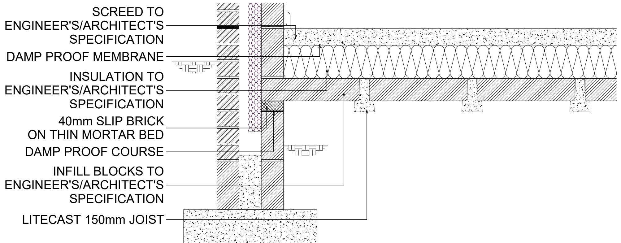
TRADITIONAL 150mm BEAM AND BLOCK SOLUTION
